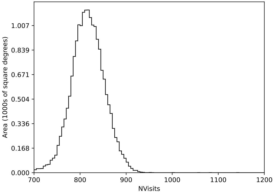
internal_u_expt45_nscale1.1v3.4_10yrs All sky all bands: NVisits
