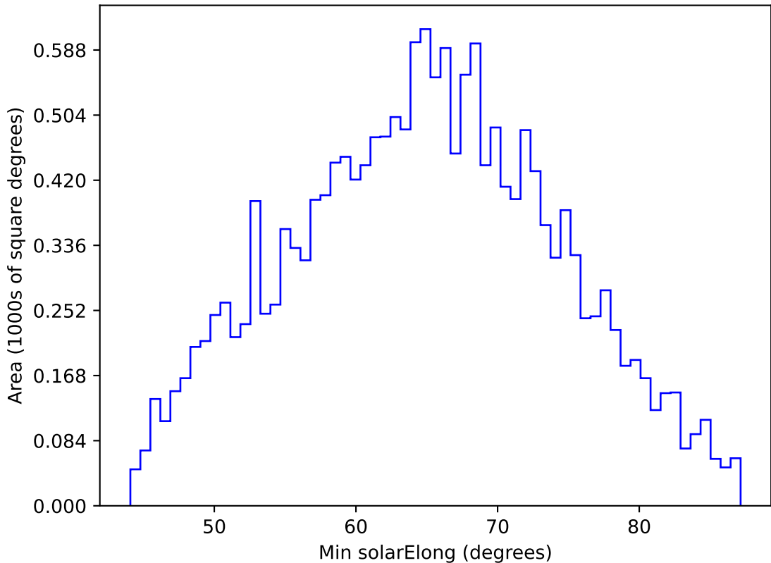
internal_u_expt45_nscale1.1v3.4_10yrs WFD y band: Min solarElong
