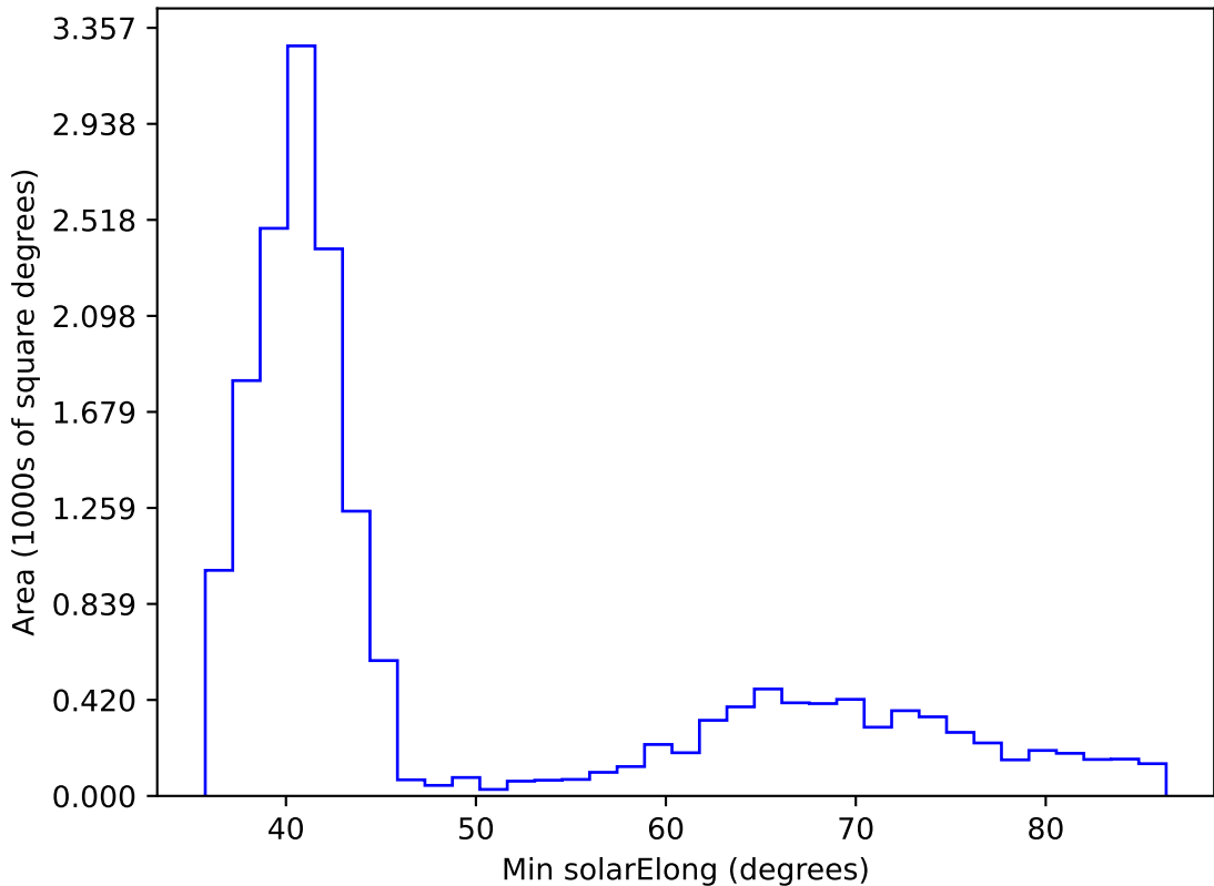
internal_u_expt45_nscale1.1v3.4_10yrs WFD i band: Min solarElong
