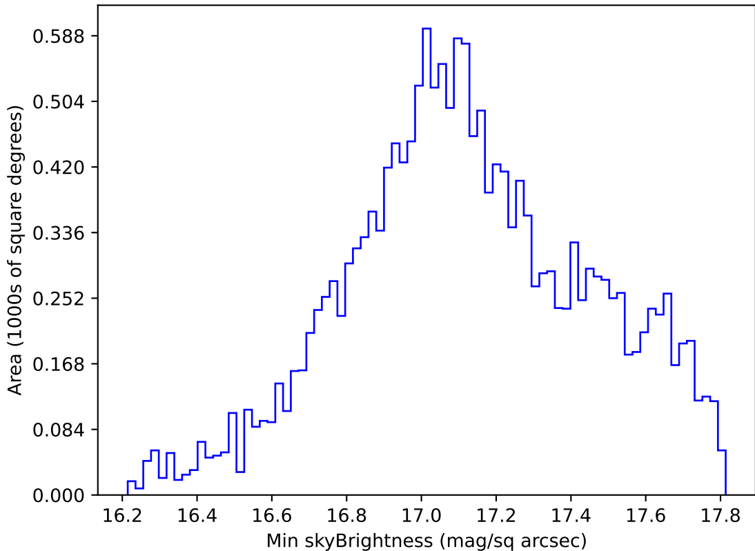
internal_u_expt45_nscale1.1v3.4_10yrs WFD y band: Min skyBrightness
