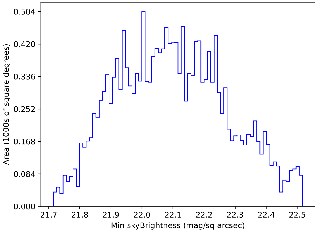
internal_u_expt45_nscale1.1v3.4_10yrs WFD u band: Min skyBrightness
