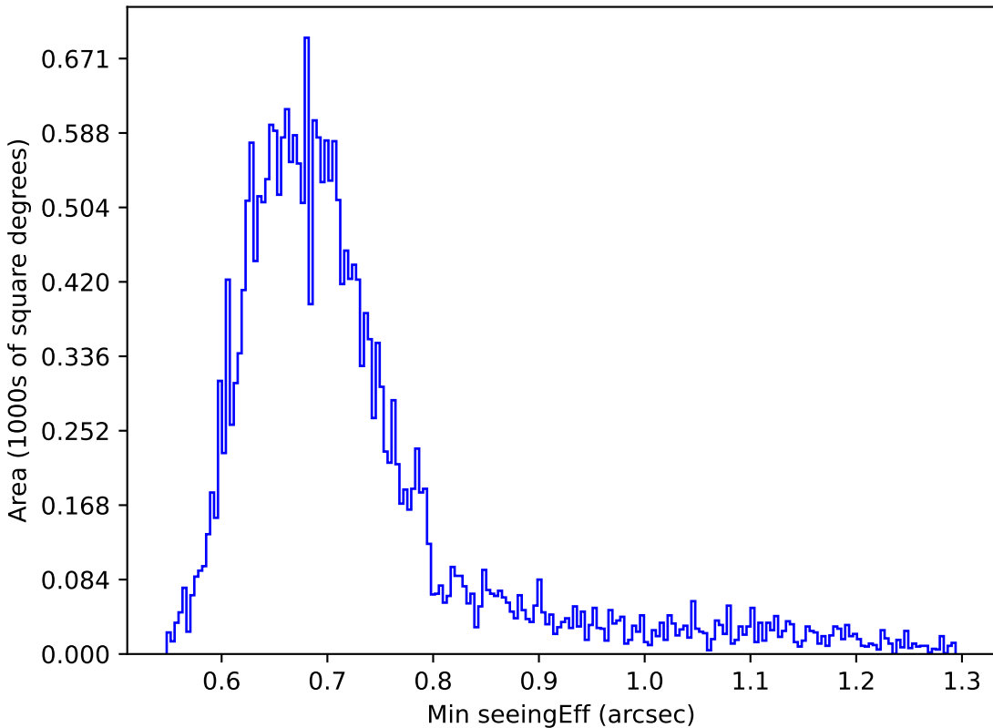
internal_u_expt45_nscale1.1v3.4_10yrs Yr 1 r band: Min seeingEff
