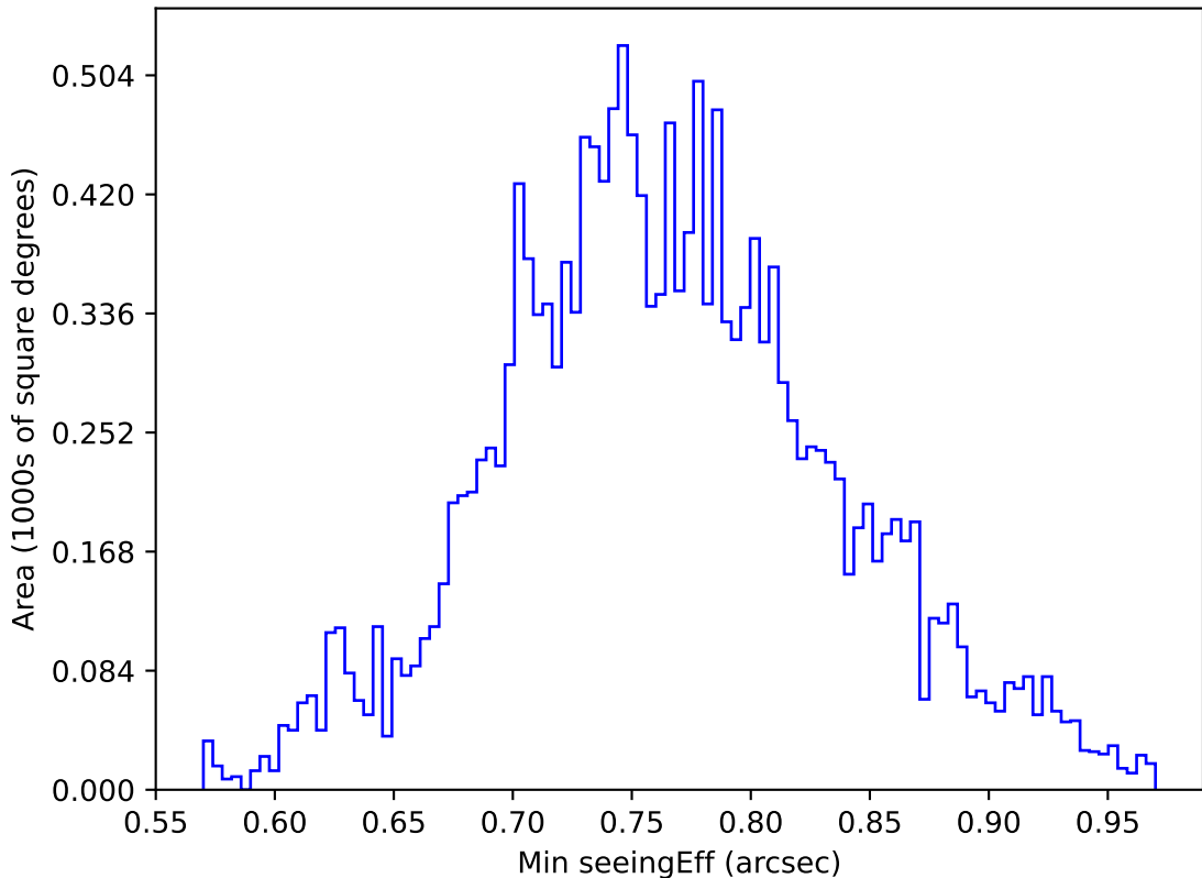
internal_u_expt45_nscale1.1v3.4_10yrs WFD u band: Min seeingEff
