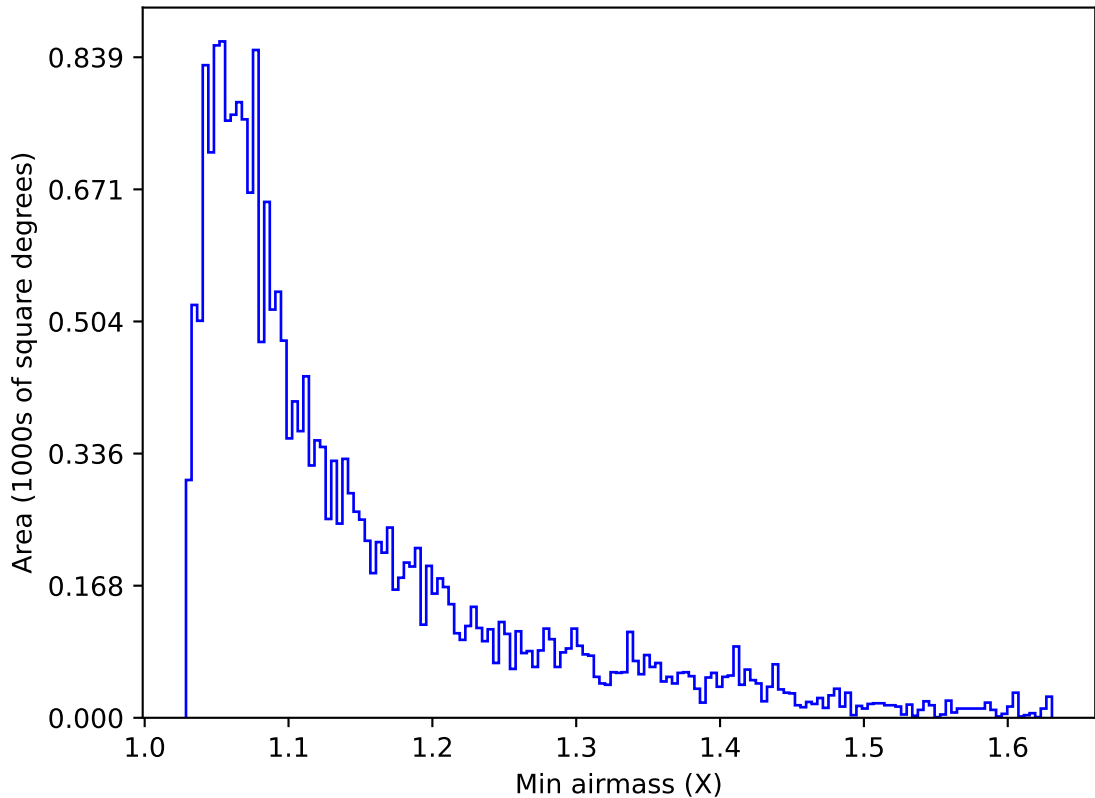
internal_u_expt45_nscale1.1v3.4_10yrs Yr 1 u band: Min airmass
