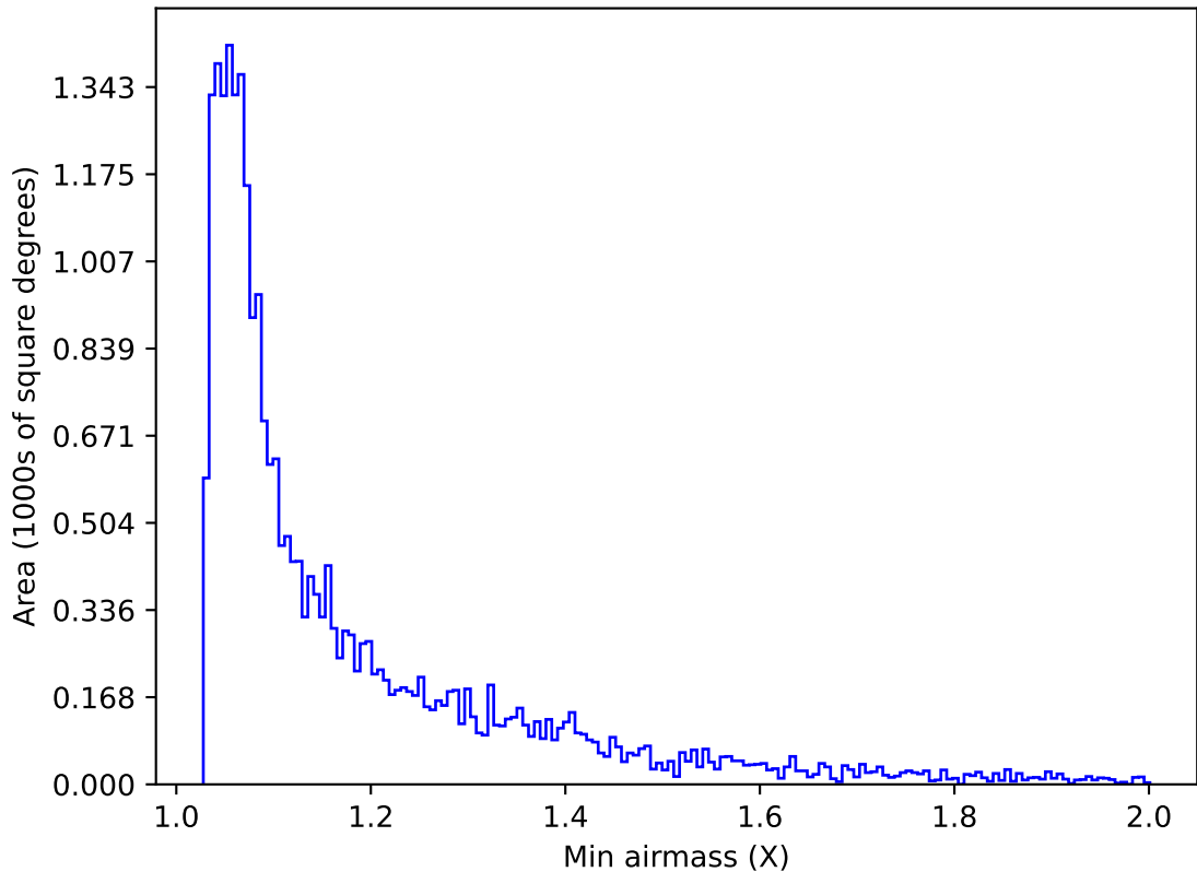
internal_u_expt45_nscale1.1v3.4_10yrs Yr 1 g band: Min airmass
