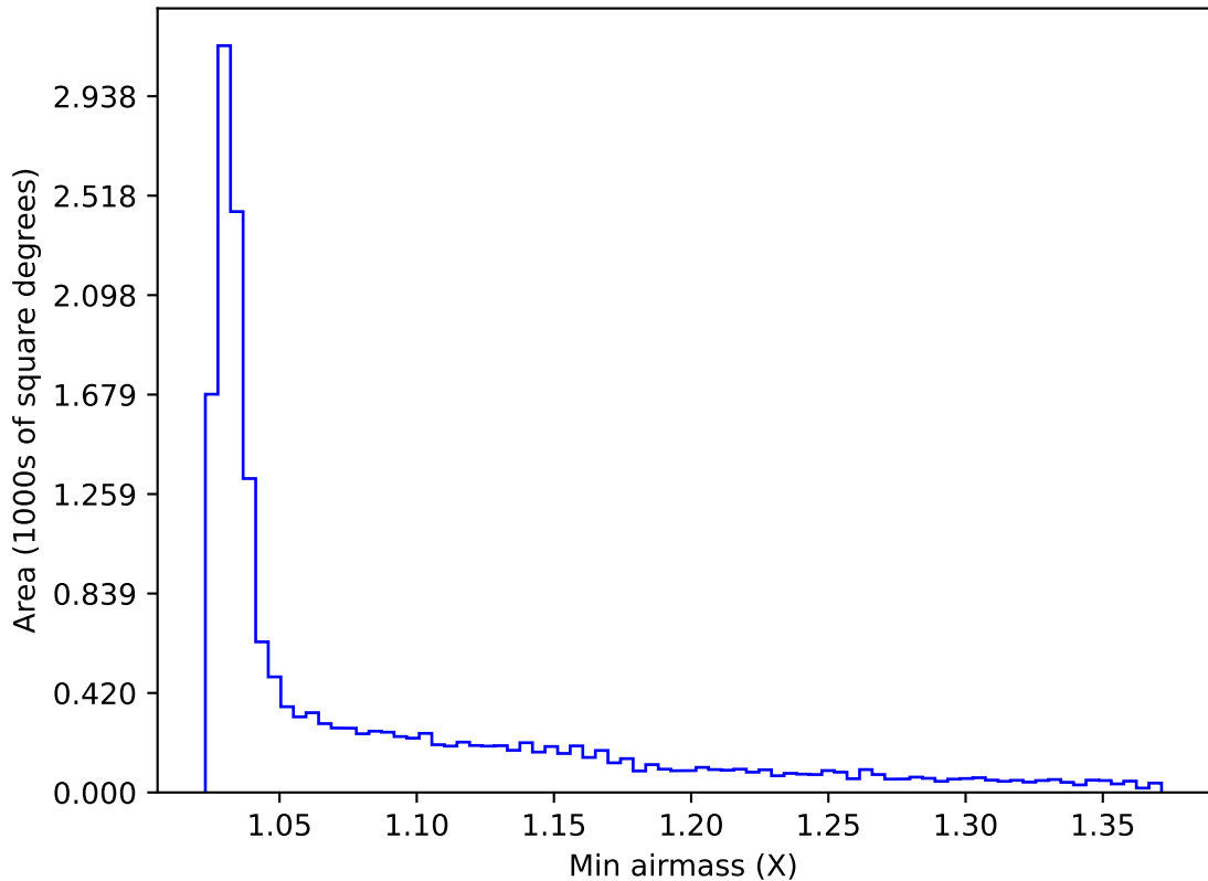
internal_u_expt45_nscale1.1v3.4_10yrs WFD y band: Min airmass
