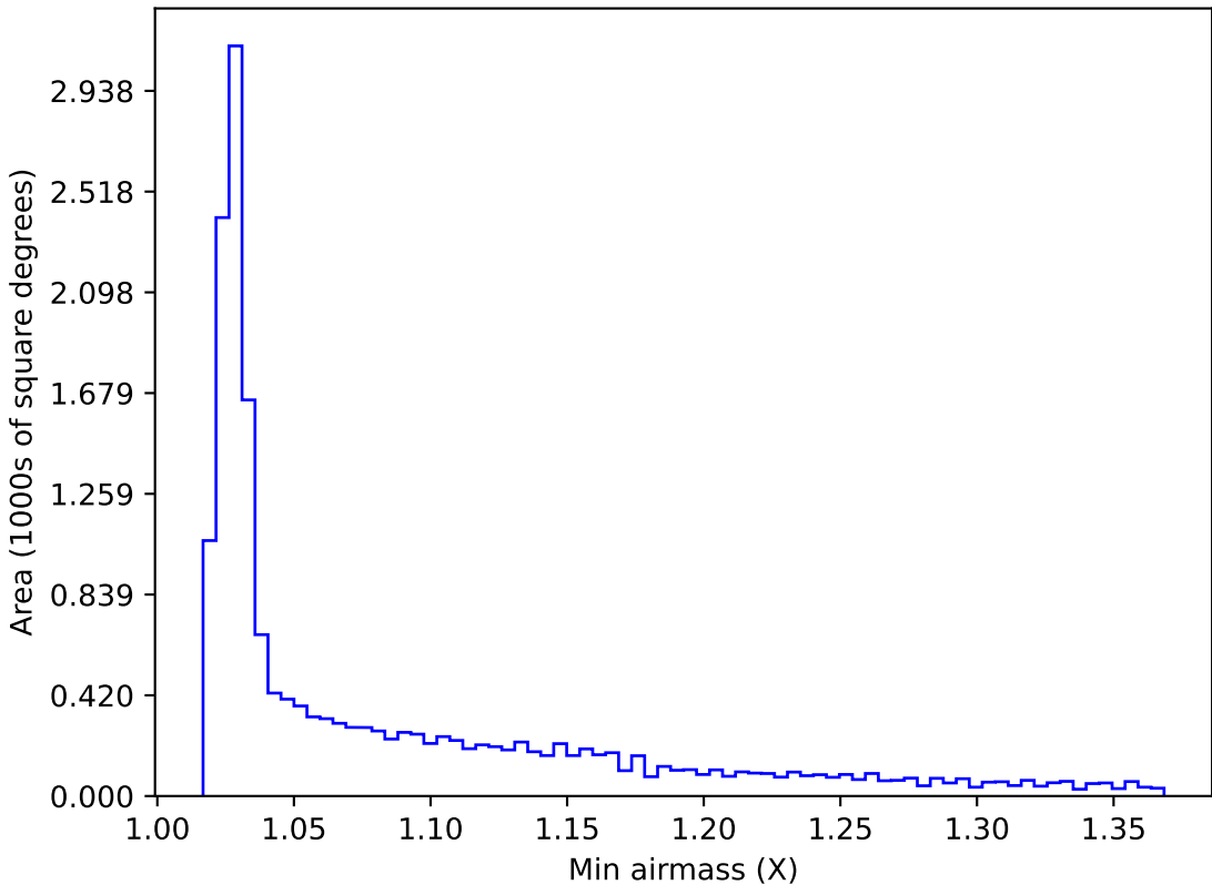
internal_u_expt45_nscale1.1v3.4_10yrs WFD r band: Min airmass
