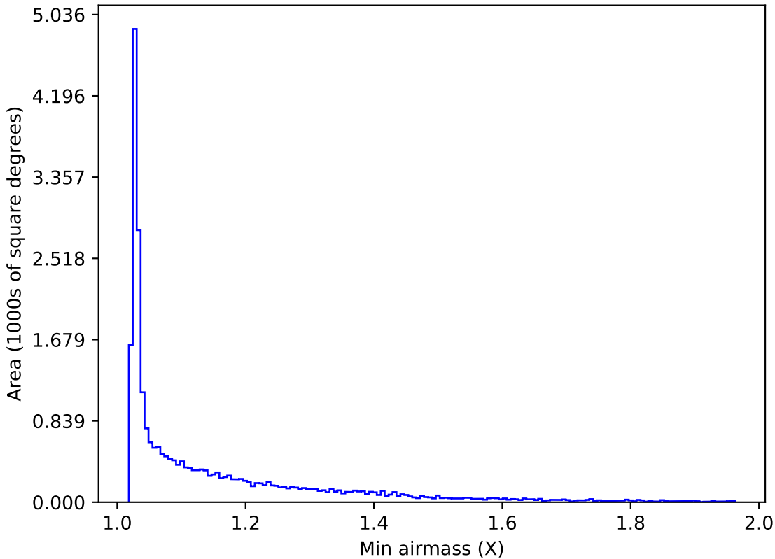
internal_u_expt45_nscale1.1v3.4_10yrs All sky i band: Min airmass
