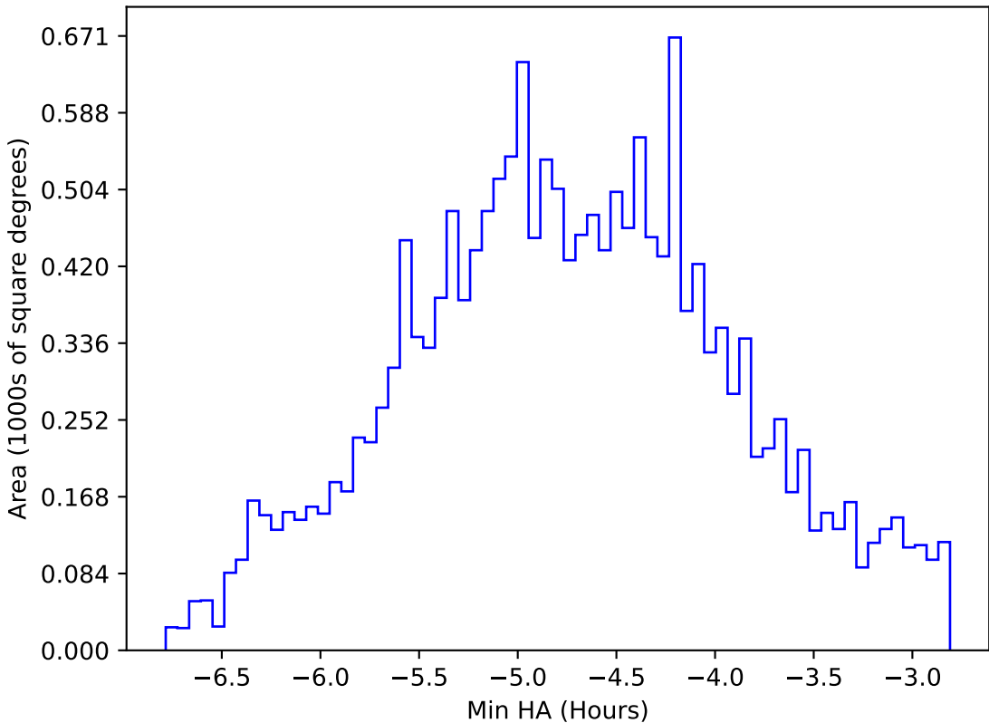
internal_u_expt45_nscale1.1v3.4_10yrs WFD all bands: Min HA
