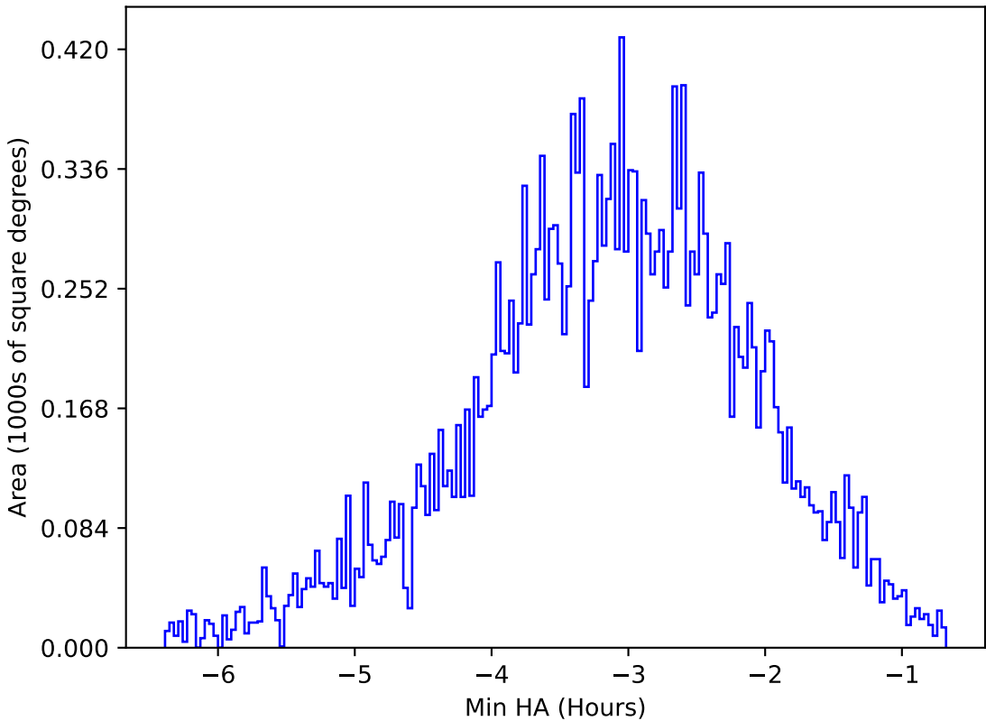
internal_u_expt45_nscale1.1v3.4_10yrs All sky u band: Min HA
