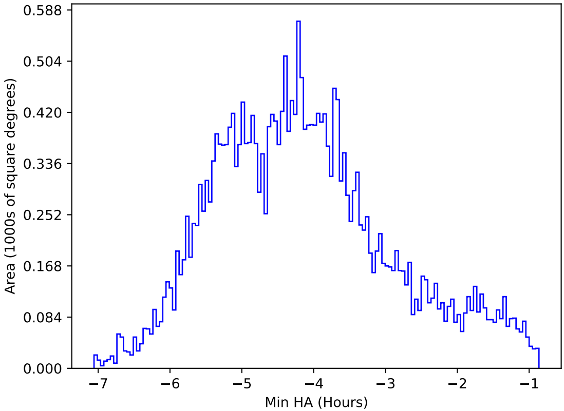
internal_u_expt45_nscale1.1v3.4_10yrs All sky r band: Min HA
