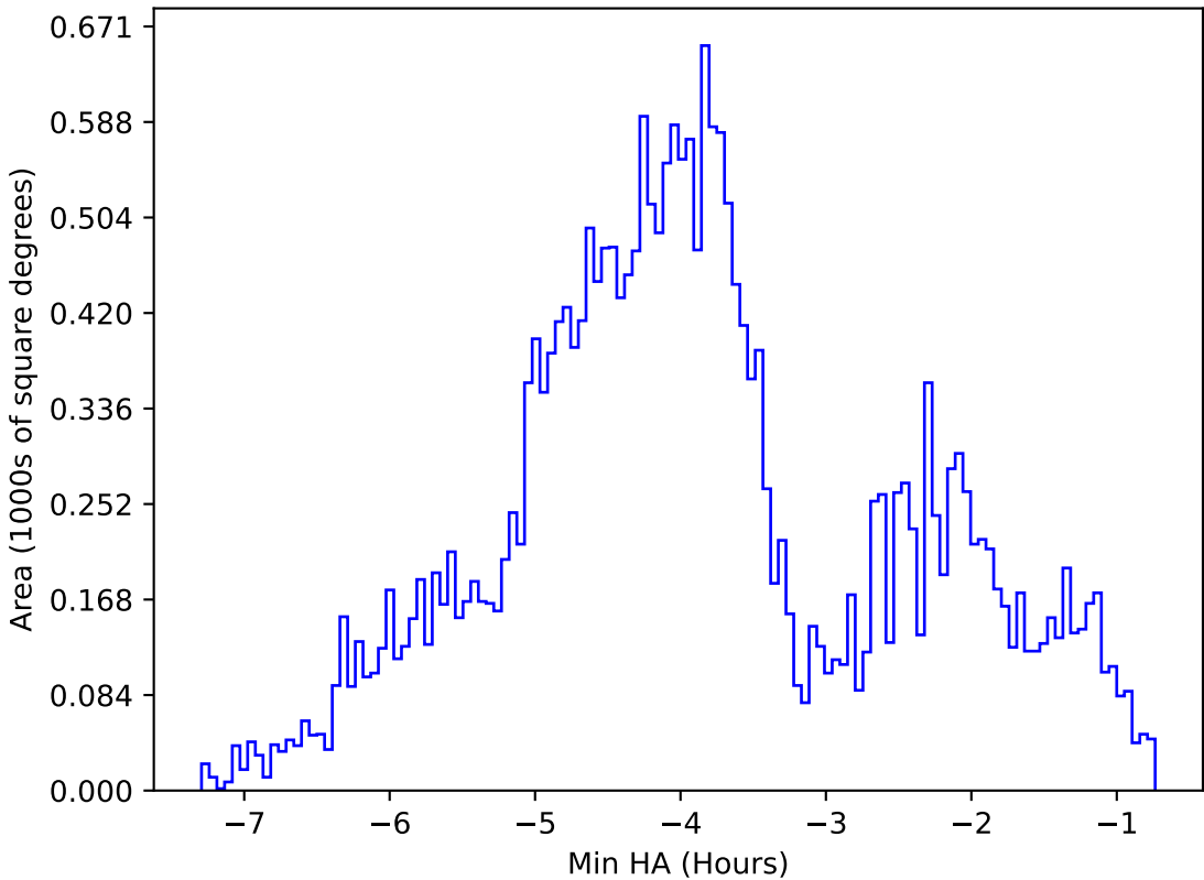
internal_u_expt45_nscale1.1v3.4_10yrs All sky g band: Min HA
