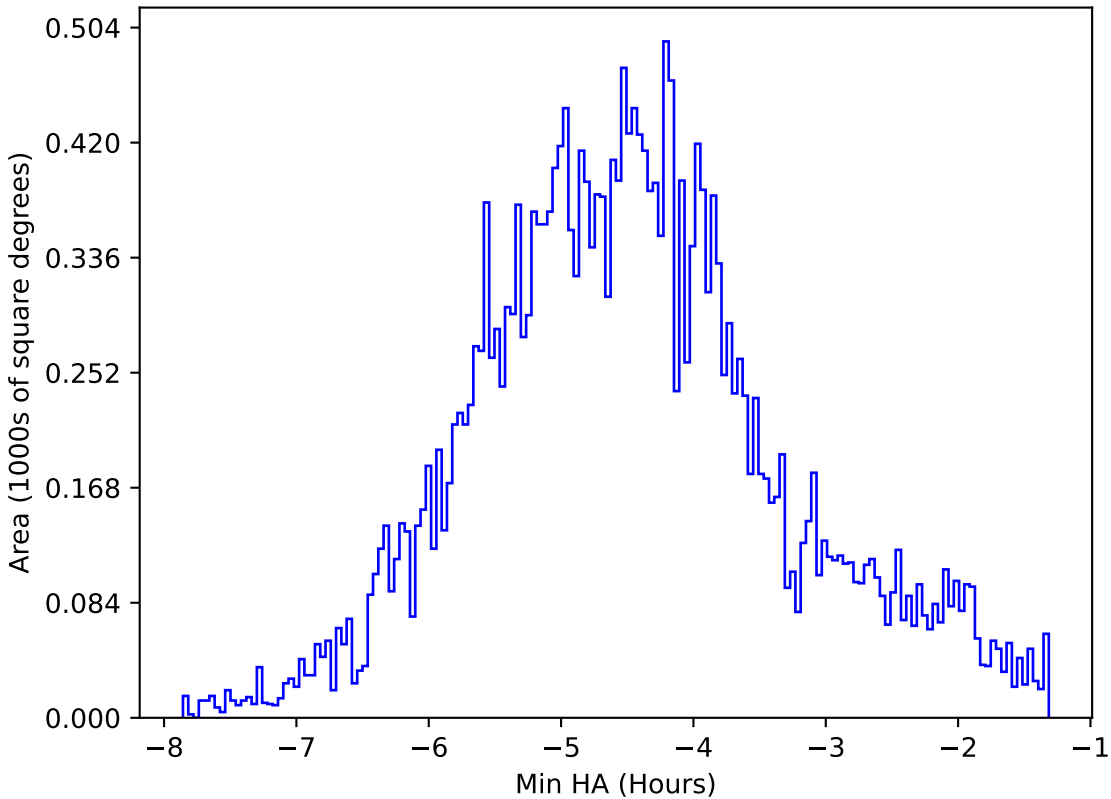
internal_u_expt45_nscale1.1v3.4_10yrs All sky all bands: Min HA
