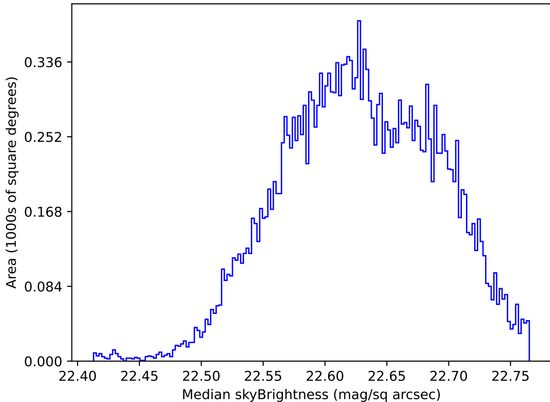
internal_u_expt45_nscale1.1v3.4_10yrs Yr 1 u band: Median skyBrightness
