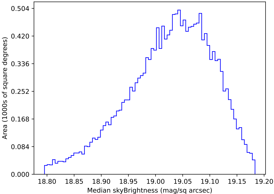
internal_u_expt45_nscale1.1v3.4_10yrs WFD z band: Median skyBrightness
