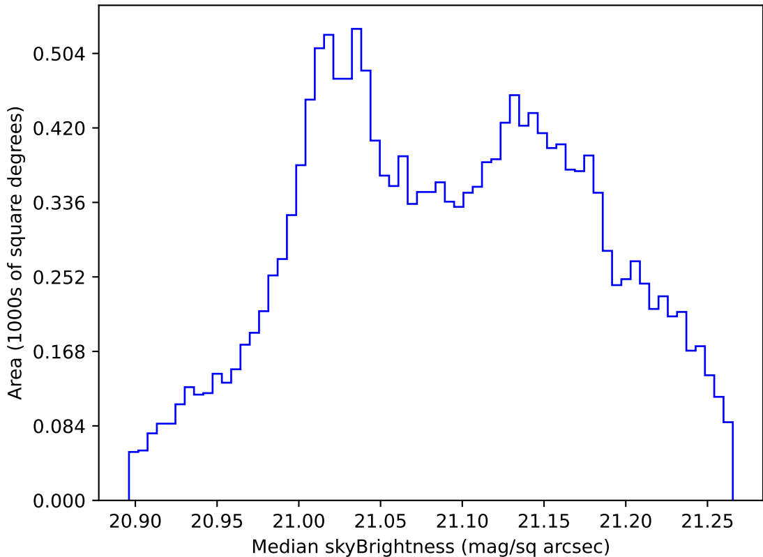
internal_u_expt45_nscale1.1v3.4_10yrs WFD r band: Median skyBrightness
