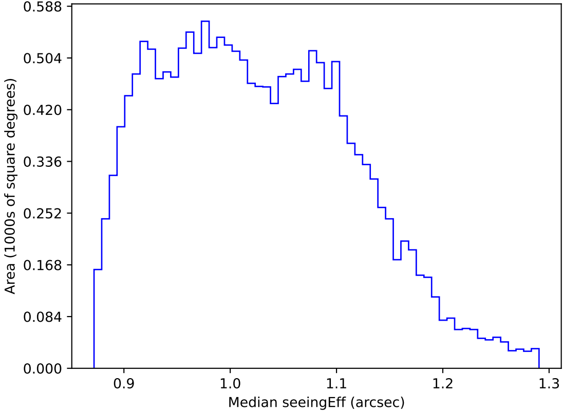
internal_u_expt45_nscale1.1v3.4_10yrs WFD r band: Median seeingEff
