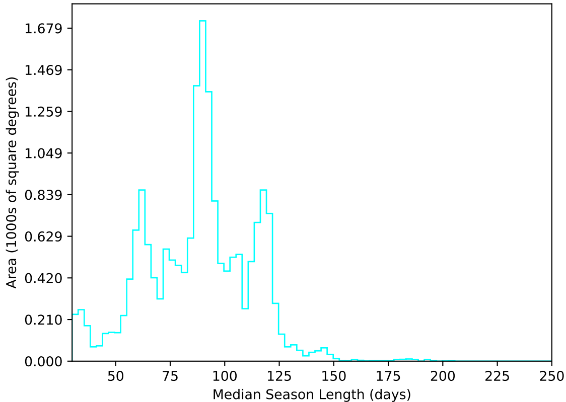
internal_u_expt45_nscale1.1v3.4_10yrs WFD u band: Median Season Length
