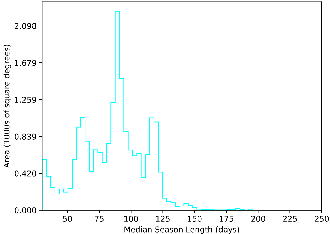
internal_u_expt45_nscale1.1v3.4_10yrs All sky u band: Median Season Length
