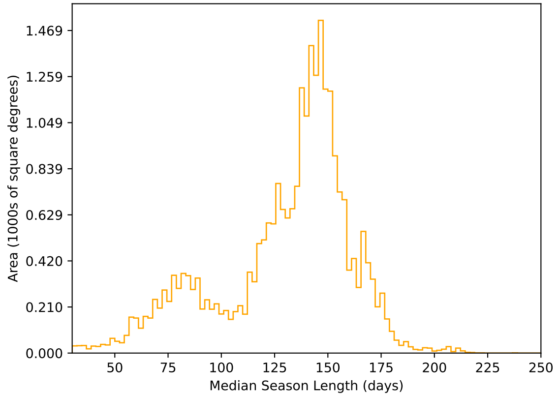
internal_u_expt45_nscale1.1v3.4_10yrs All sky r band: Median Season Length
