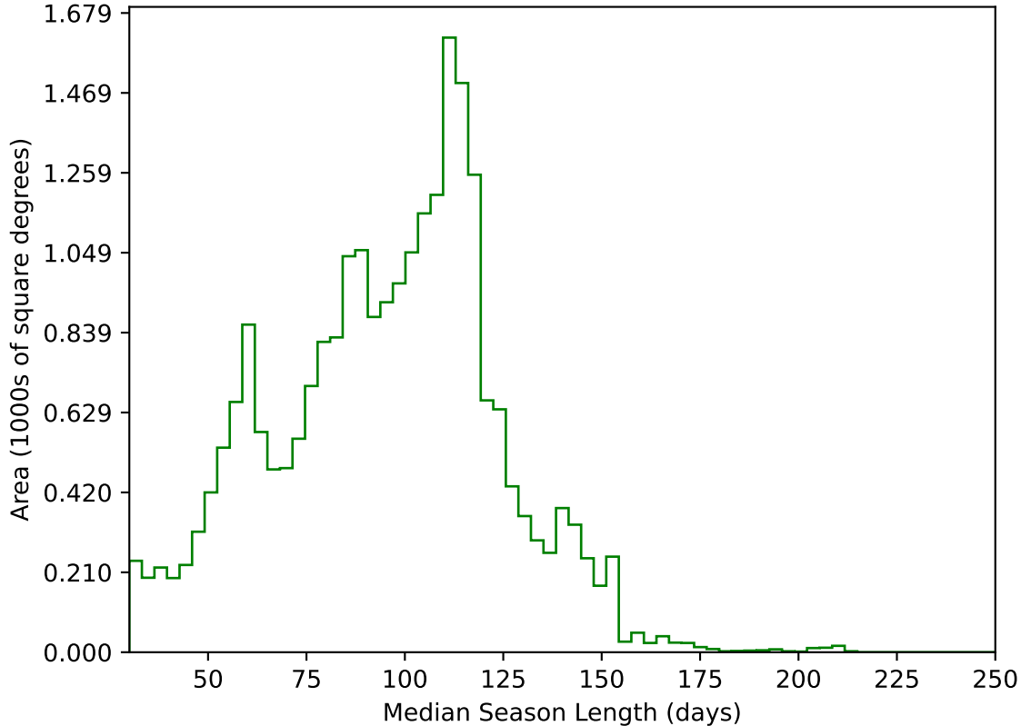
internal_u_expt45_nscale1.1v3.4_10yrs All sky g band: Median Season Length
