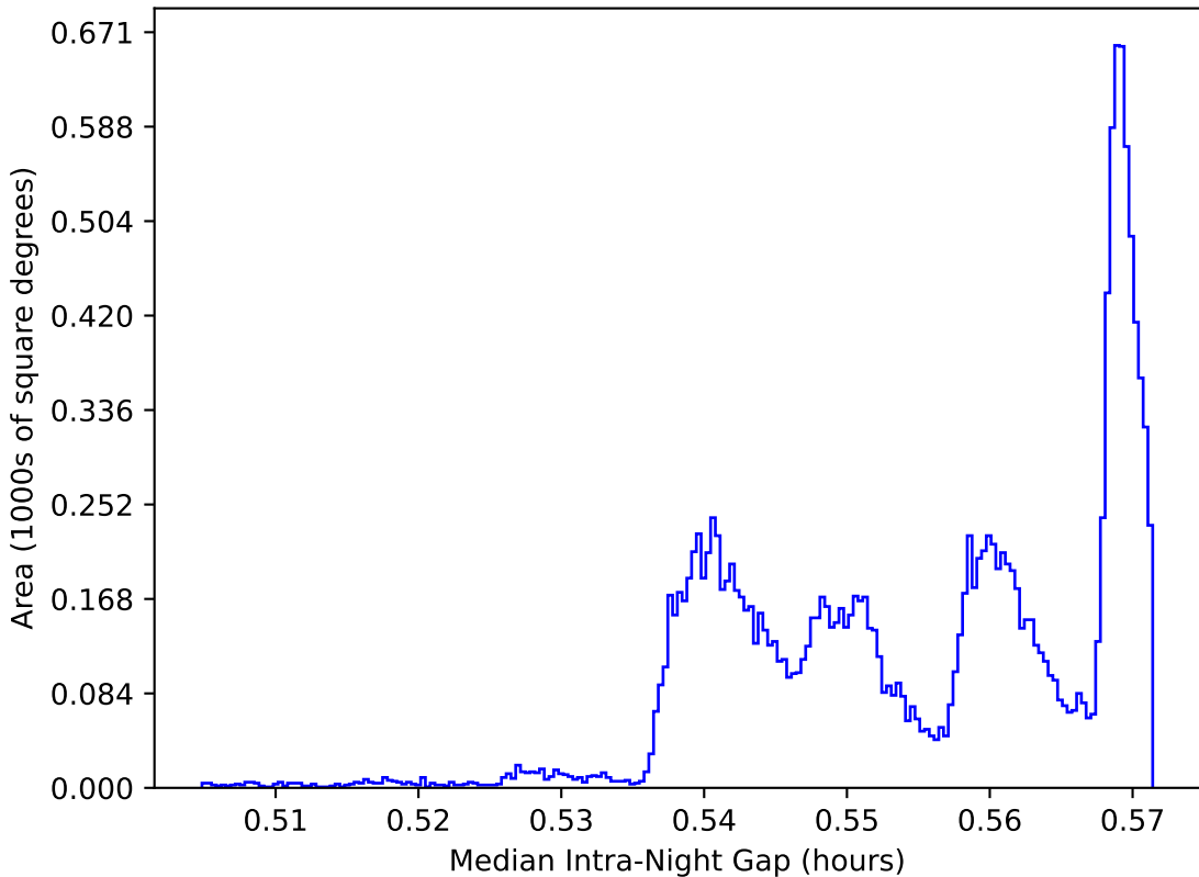
internal_u_expt45_nscale1.1v3.4_10yrs WFD: Median Intra-Night Gap
