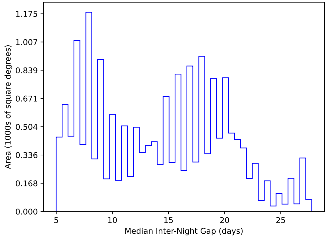
internal_u_expt45_nscale1.1v3.4_10yrs WFD y band: Median Inter-Night Gap
