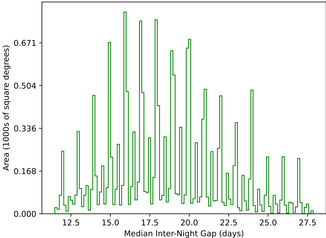
internal_u_expt45_nscale1.1v3.4_10yrs WFD g band: Median Inter-Night Gap
