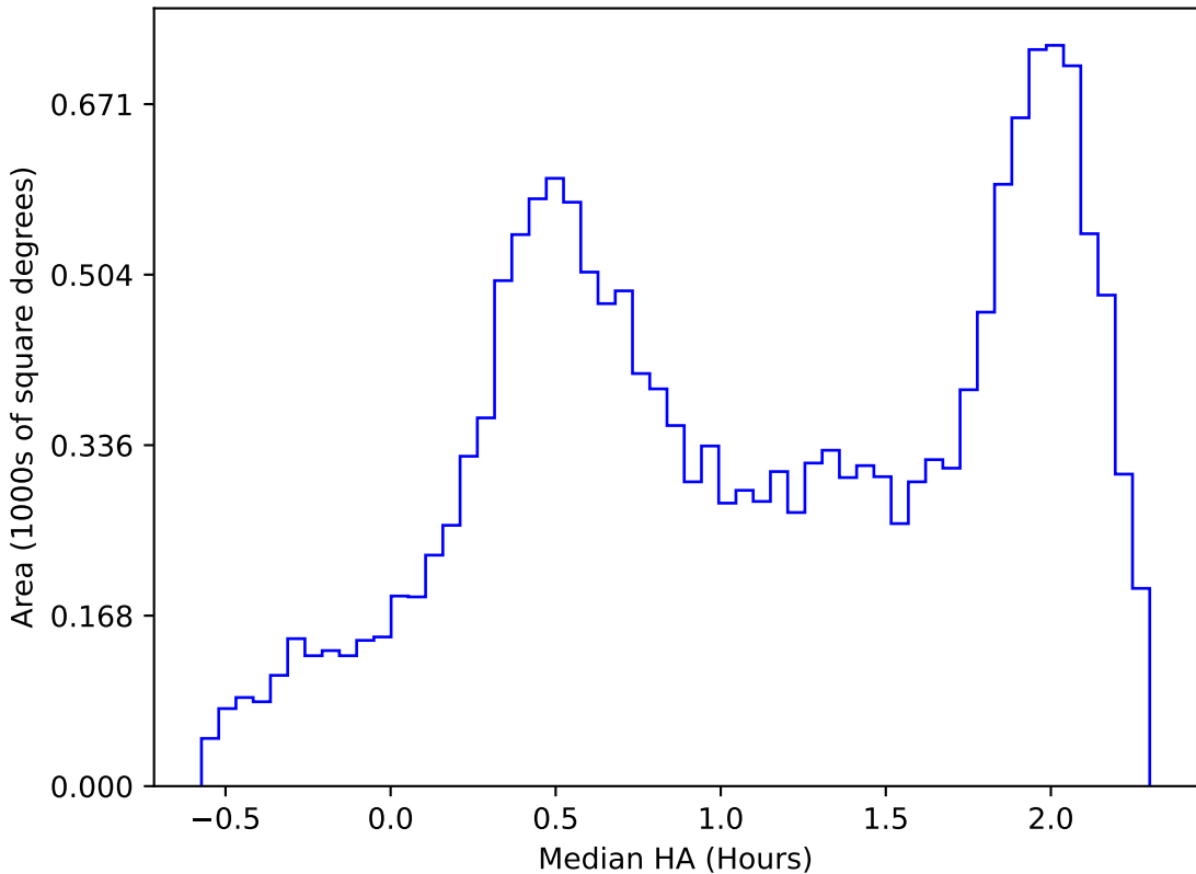
internal_u_expt45_nscale1.1v3.4_10yrs WFD z band: Median HA
