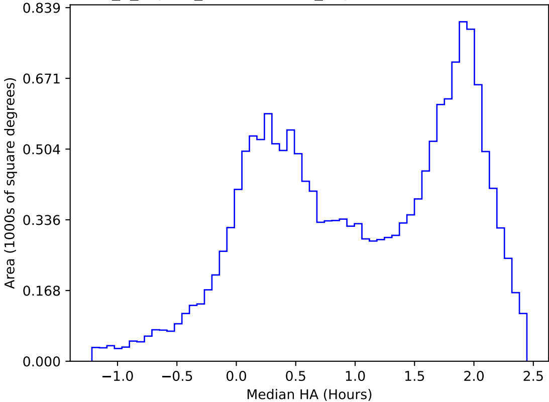
internal_u_expt45_nscale1.1v3.4_10yrs WFD u band: Median HA
