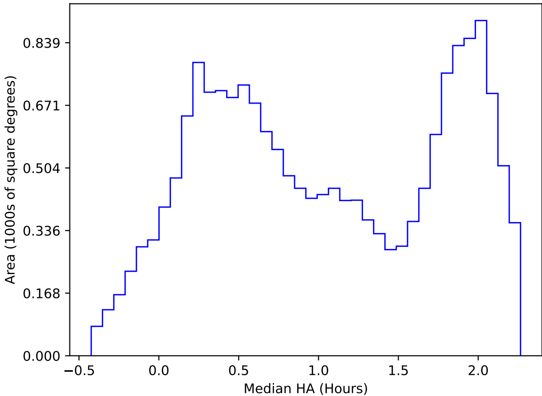
internal_u_expt45_nscale1.1v3.4_10yrs WFD i band: Median HA
