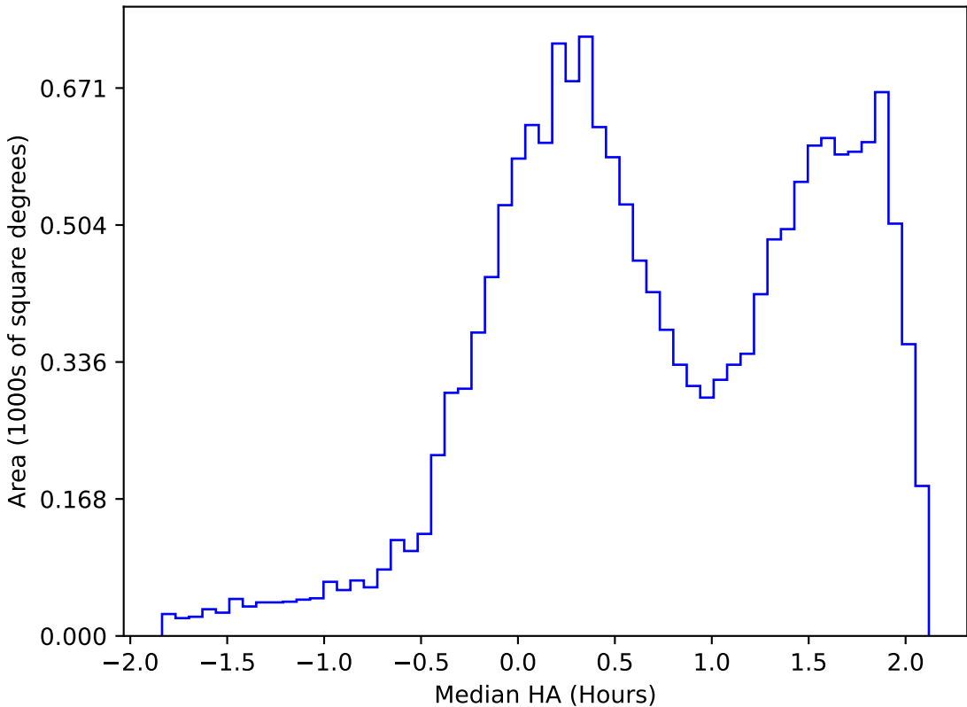
internal_u_expt45_nscale1.1v3.4_10yrs WFD g band: Median HA
