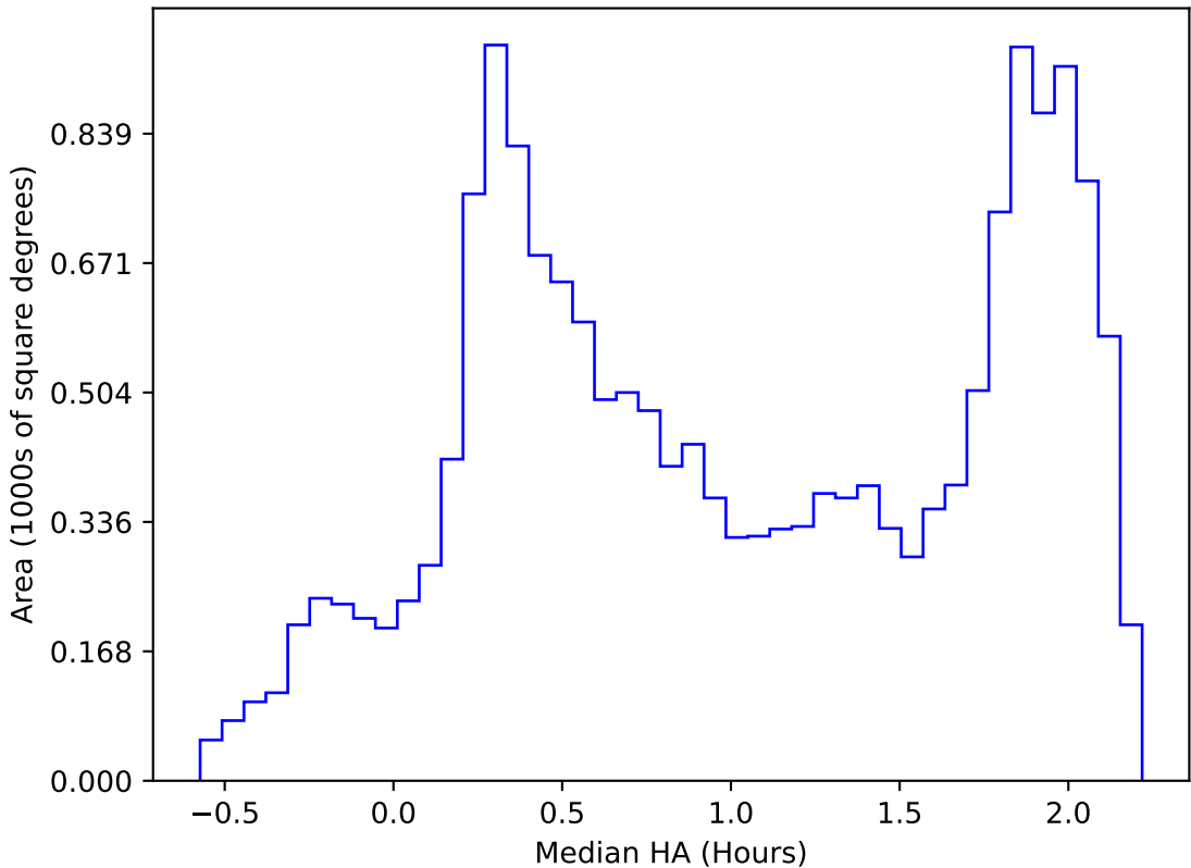
internal_u_expt45_nscale1.1v3.4_10yrs WFD all bands: Median HA
