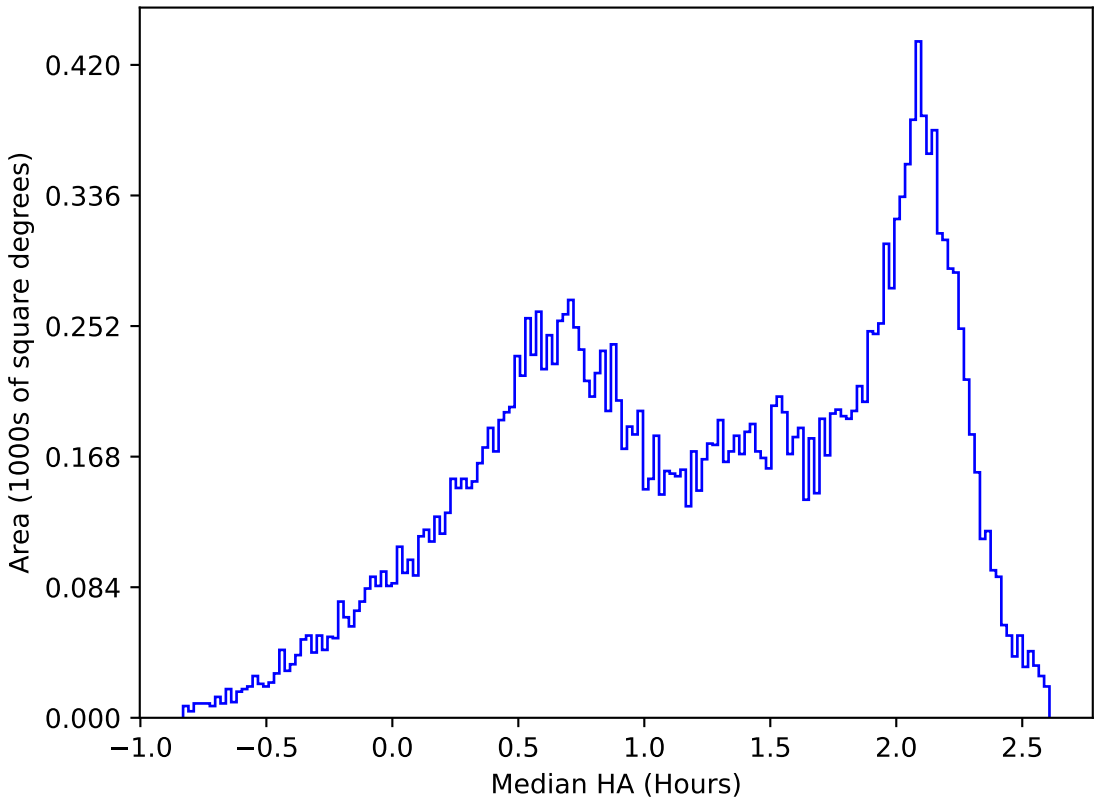
internal_u_expt45_nscale1.1v3.4_10yrs All sky y band: Median HA
