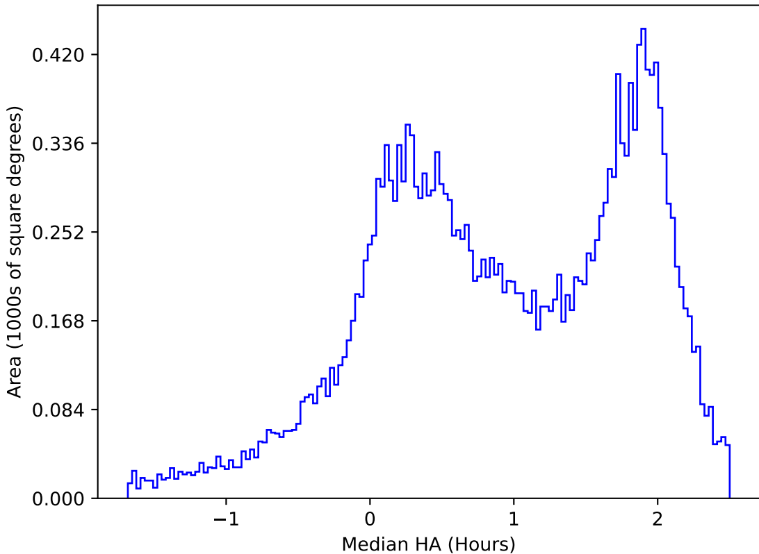
internal_u_expt45_nscale1.1v3.4_10yrs All sky u band: Median HA
