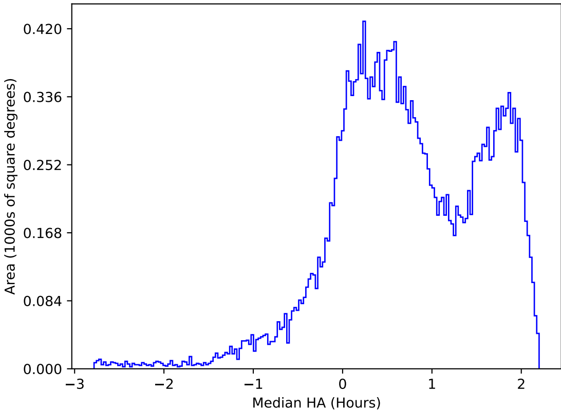
internal_u_expt45_nscale1.1v3.4_10yrs All sky r band: Median HA
