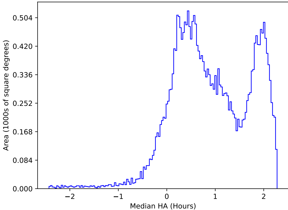
internal_u_expt45_nscale1.1v3.4_10yrs All sky i band: Median HA
