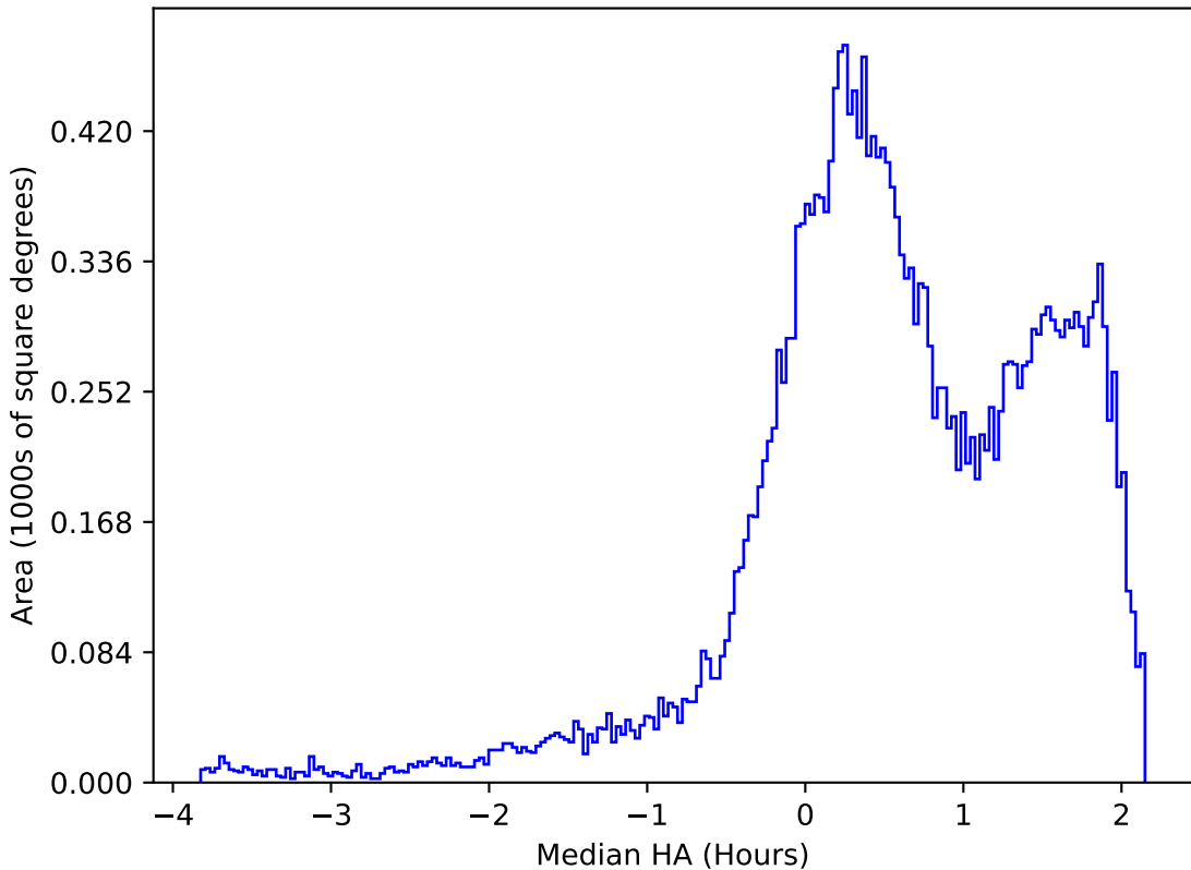
internal_u_expt45_nscale1.1v3.4_10yrs All sky g band: Median HA
