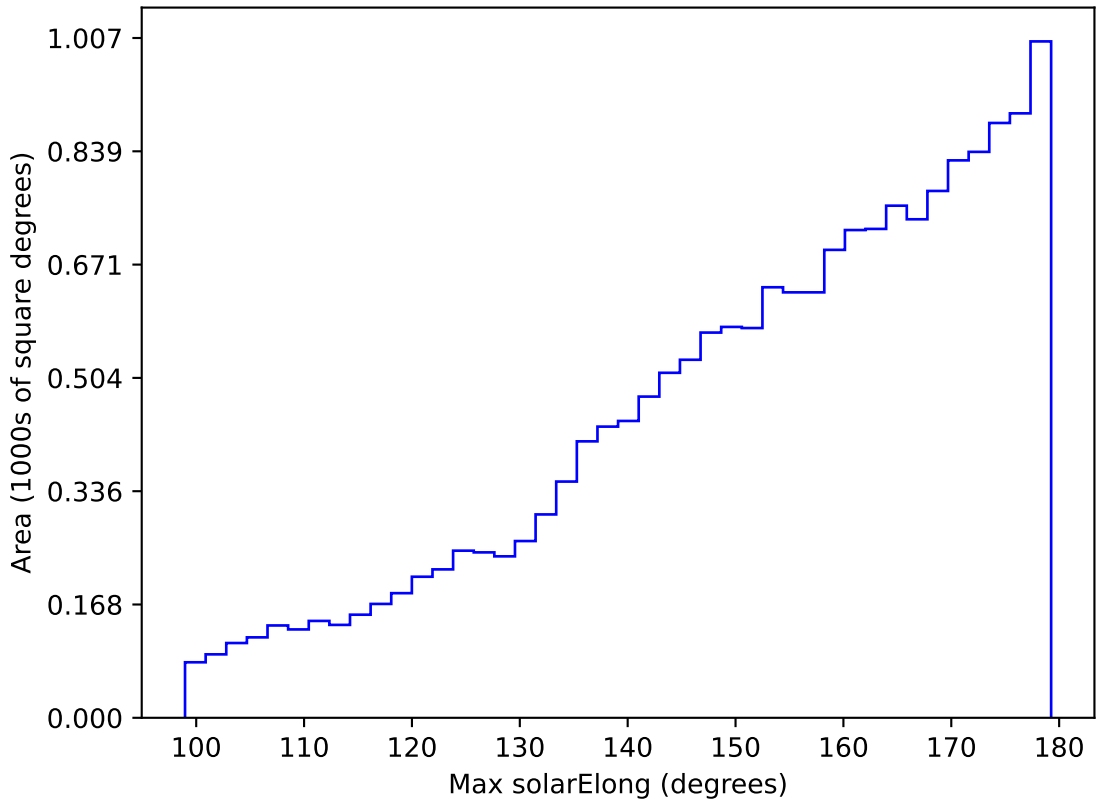
internal_u_expt45_nscale1.1v3.4_10yrs WFD y band: Max solarElong
