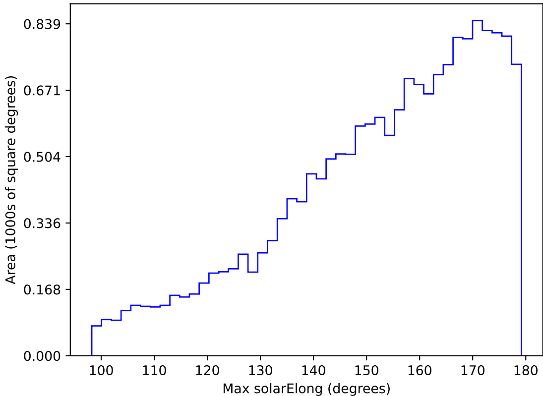
internal_u_expt45_nscale1.1v3.4_10yrs WFD u band: Max solarElong
