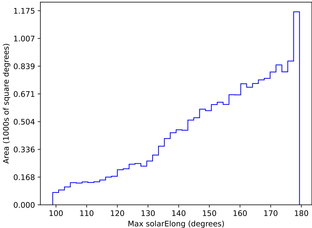
internal_u_expt45_nscale1.1v3.4_10yrs WFD i band: Max solarElong
