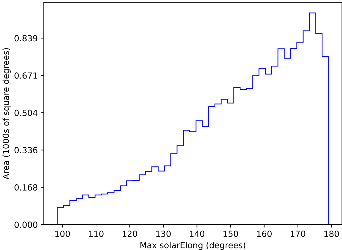
internal_u_expt45_nscale1.1v3.4_10yrs WFD g band: Max solarElong
