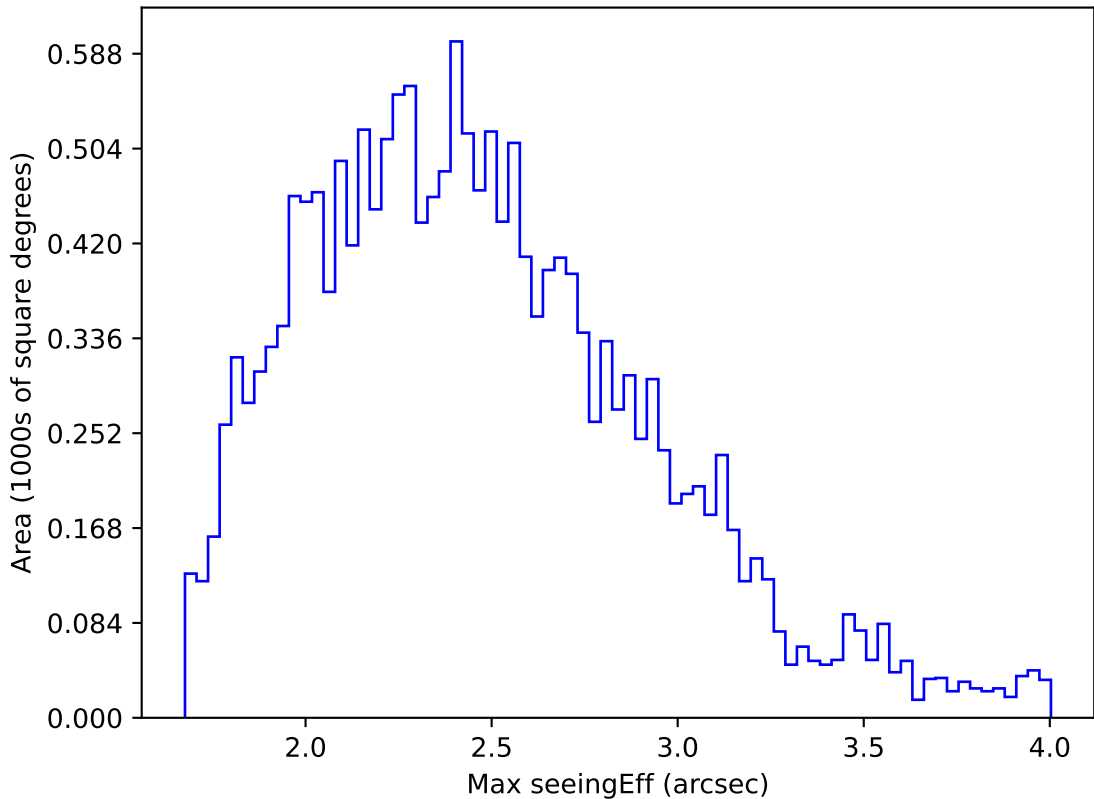
internal_u_expt45_nscale1.1v3.4_10yrs WFD g band: Max seeingEff
