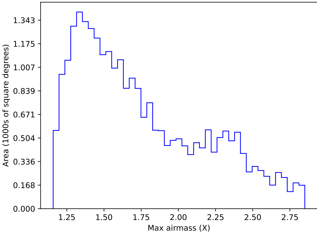
internal_u_expt45_nscale1.1v3.4_10yrs Yr 1 z band: Max airmass
