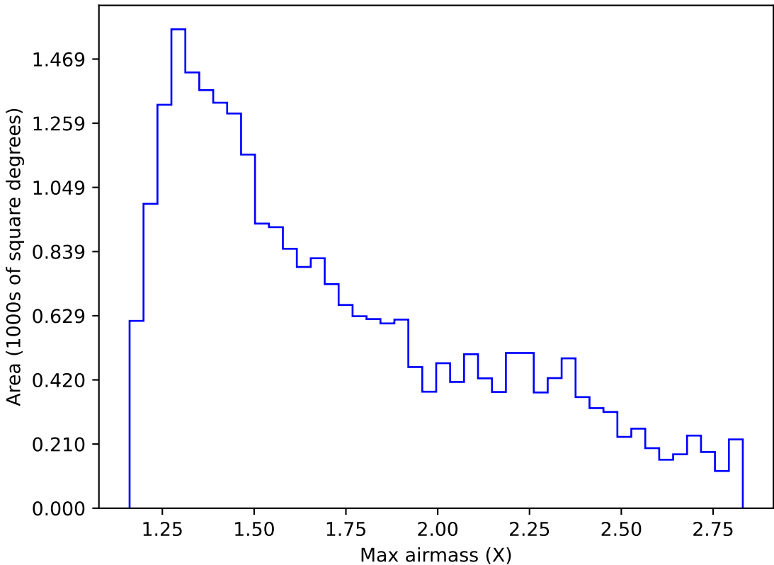
internal_u_expt45_nscale1.1v3.4_10yrs Yr 1 i band: Max airmass
