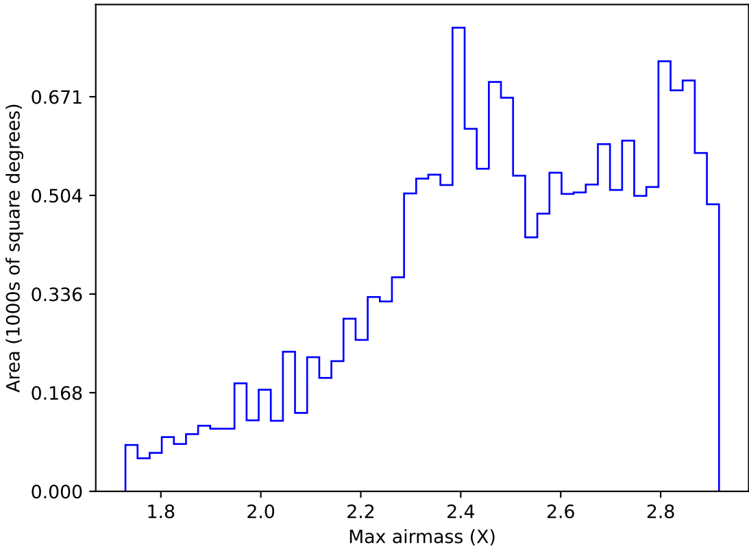
internal_u_expt45_nscale1.1v3.4_10yrs WFD z band: Max airmass
