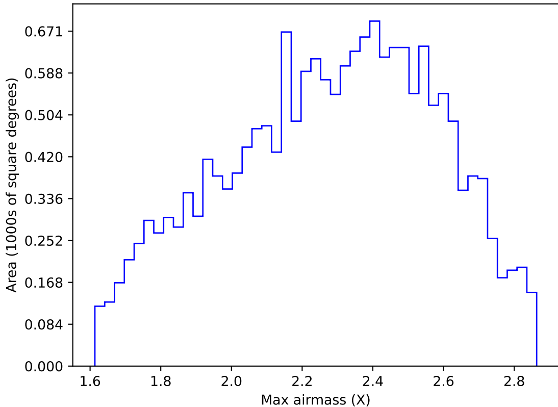
internal_u_expt45_nscale1.1v3.4_10yrs WFD y band: Max airmass
