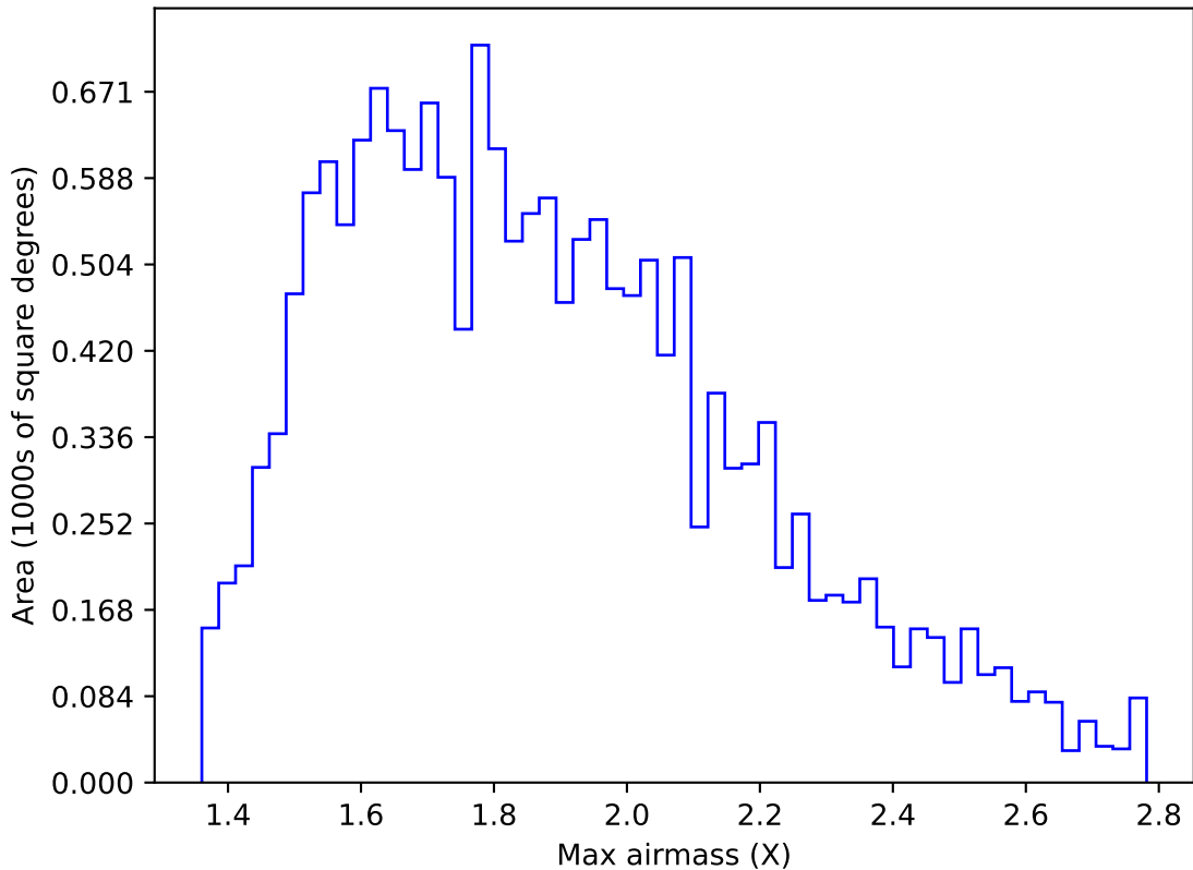
internal_u_expt45_nscale1.1v3.4_10yrs WFD u band: Max airmass
