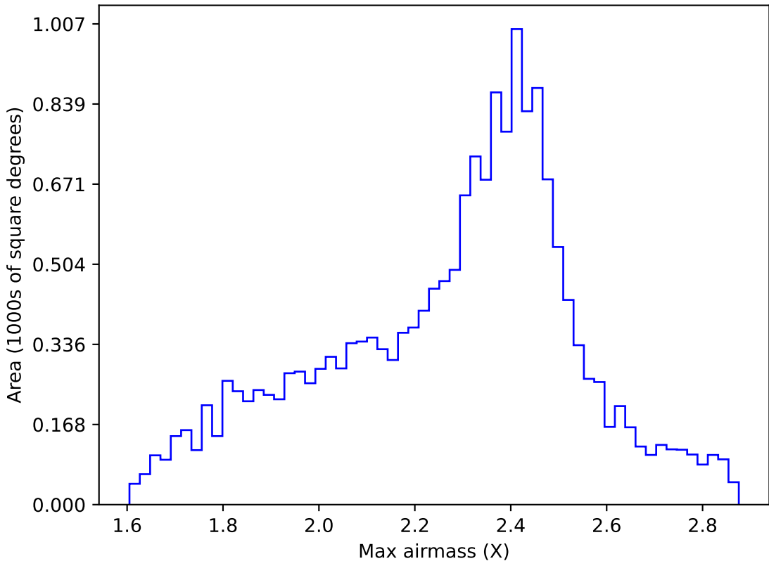
internal_u_expt45_nscale1.1v3.4_10yrs WFD r band: Max airmass
