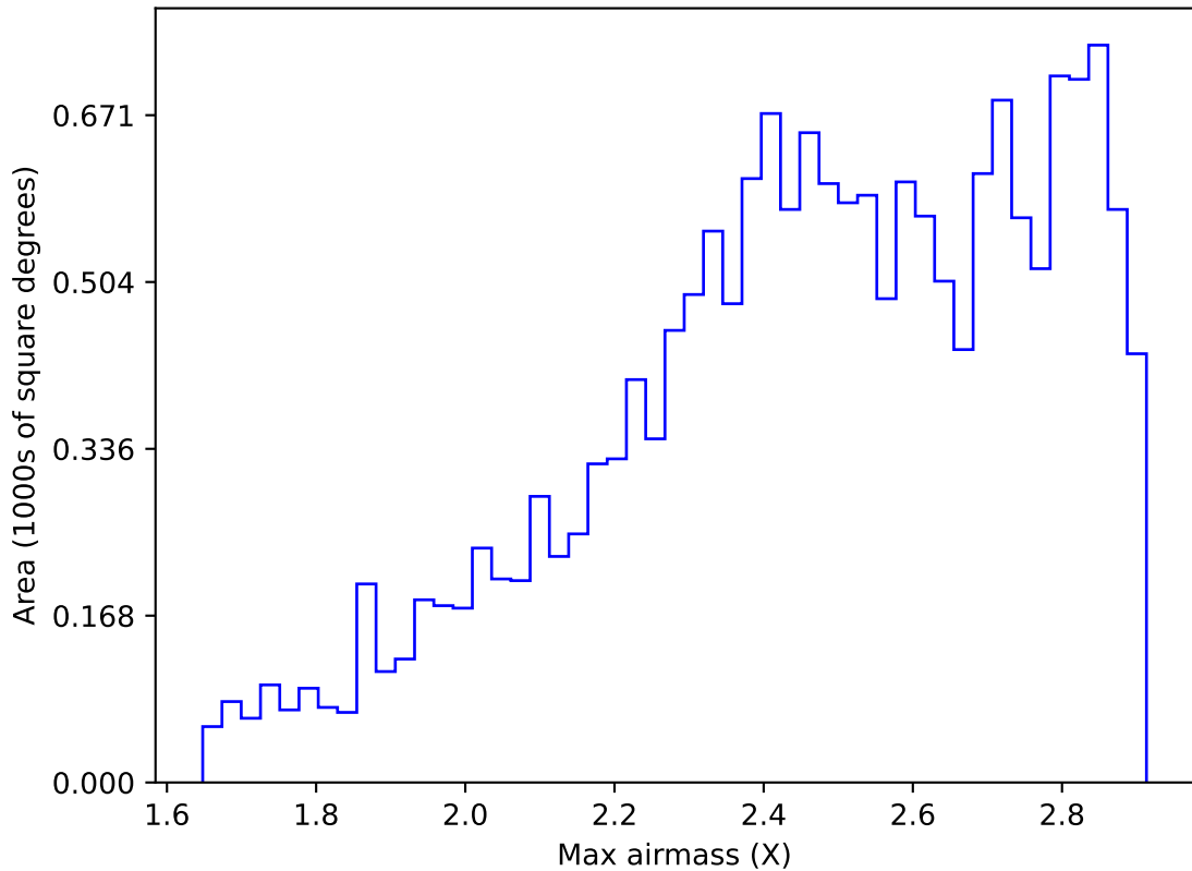
internal_u_expt45_nscale1.1v3.4_10yrs WFD i band: Max airmass
